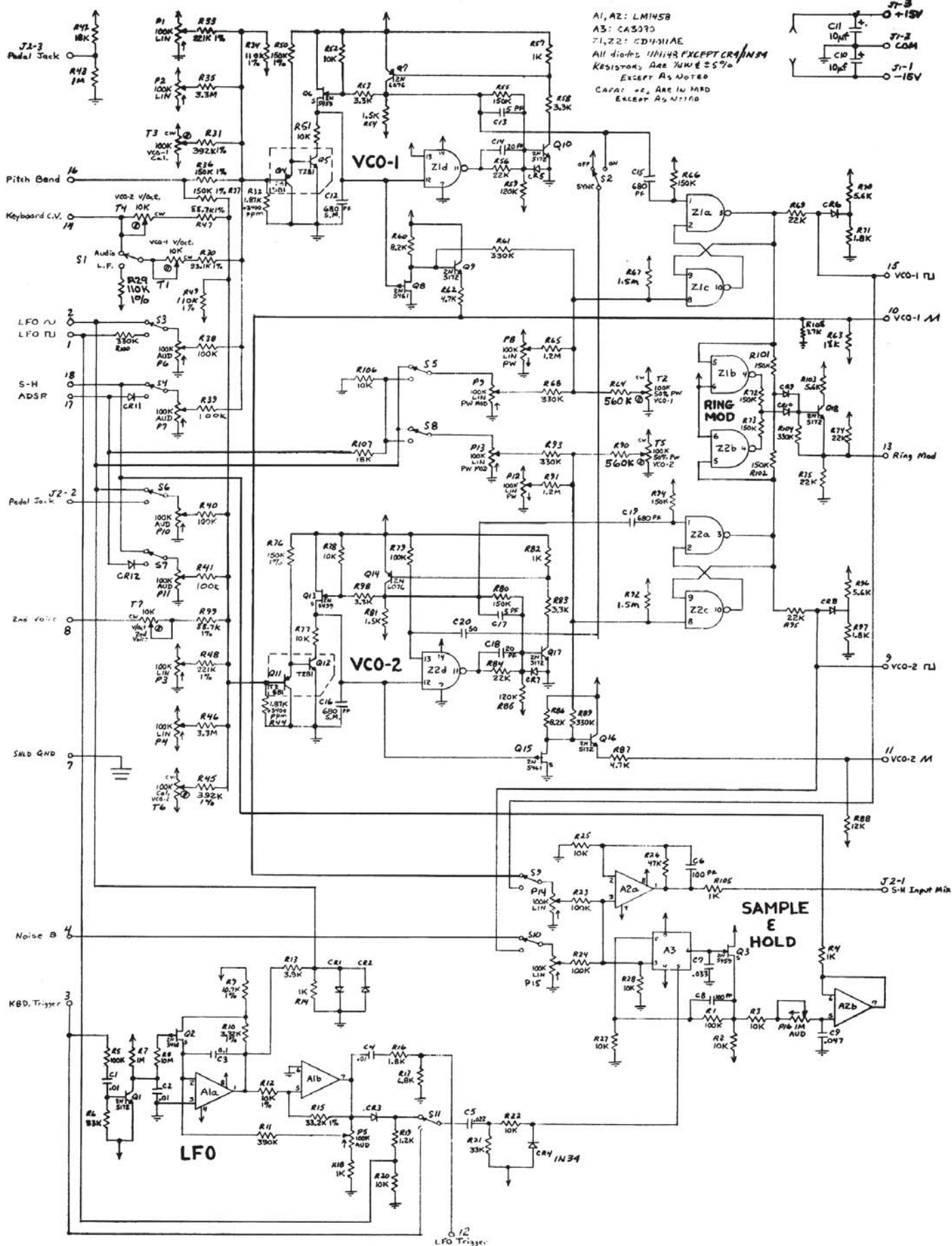
ARP ODYSSEY Model 2800 SCHEMATIC Board B-I
