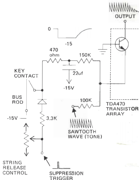
TYPICAL KEYING & GATING CIRCUIT
